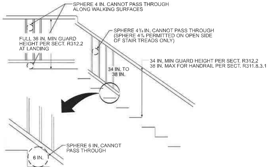
Figure R312.1.3 GUARD REQUIREMENTS
