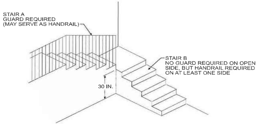
Figure R312.1.2(1) STAIRWAY GUARD
